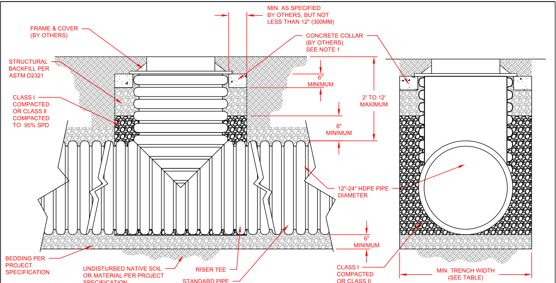
RECOMMENDED MINIMUM TRENCH WIDTHS
